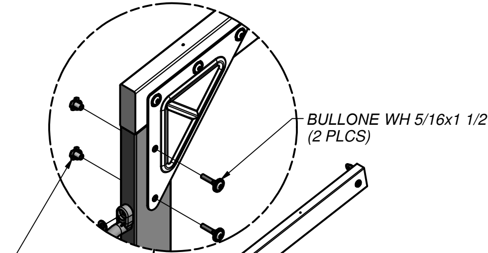
T-DADO 5/16 (2 PLCS)
