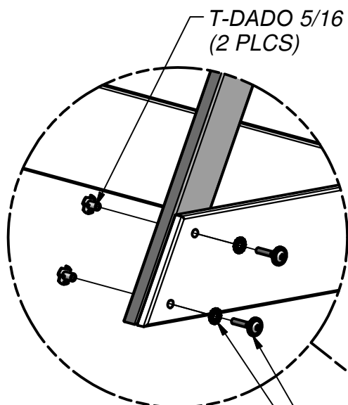
CHIUSURA RONDELLA EXT 8x19 (2 PLCS) BULLONE WH 5/16x1 1/2 (2 PLCS)
